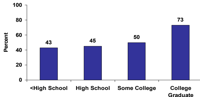
Figure 17. Percentage of adult former smokers among adult ever smokers, by educational attainment, Georgia, 2007
