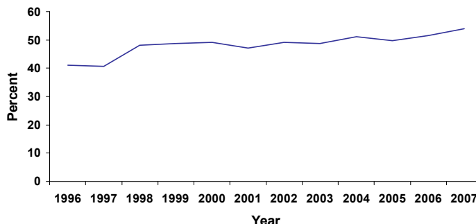
Figure 15. Proportion of former smokers among ever smokers, Georgia, 1996-2007
